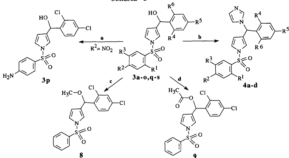
SCHEME 2
